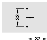
Drilling pattern
